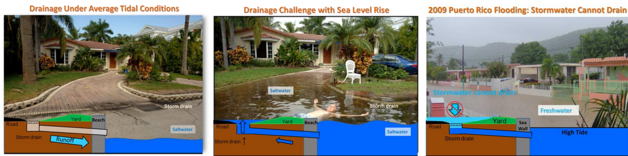
Figure 5 Gravity stormwater drainage under average tidal conditions, with sea level rise, and when combined with extreme precipitation events. (Photos 1 and 2 courtesy of the Broward County Government, Florida)
